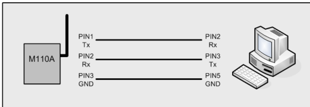
Figure 21. Hardware connection-3
